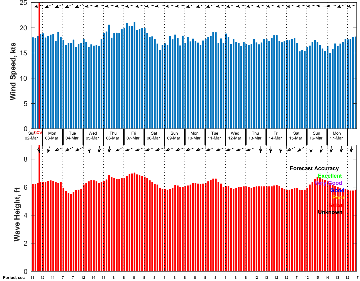
Wind & Wave Forecast for NDBC 52213 from 01-Mar-2025 11:00:00 to 17-Mar-2025 11:00:00
