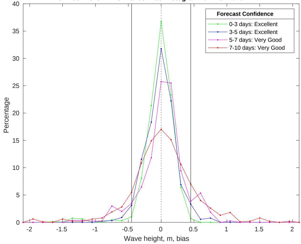
NDBC 41004 vs CMEMS Waves Bias Histogram: 02-Mar-2025
