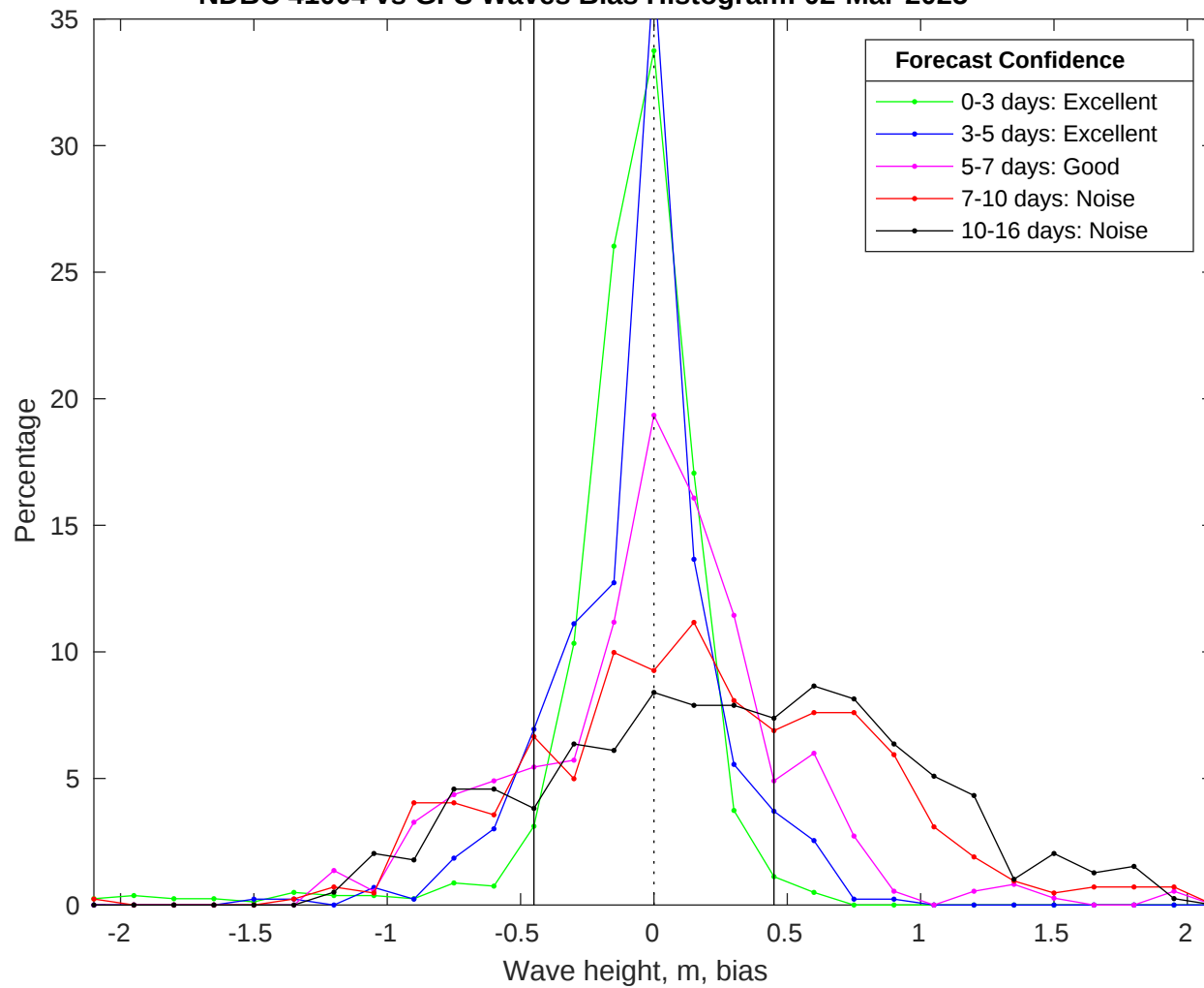
NDBC 41004 vs GFS Waves Bias Histogram: 02-Mar-2025
