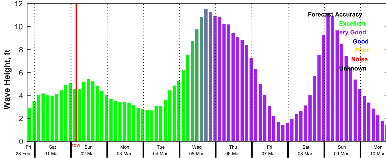
CMEMS Wave Forecast for NDBC 41004 from 28-Feb-2025 19:00:00 to 10-Mar-2025 19:00:00
