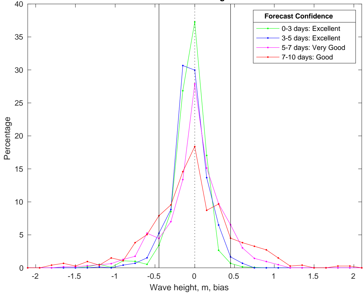
NDBC 41013 vs CMEMS Waves Bias Histogram: 02-Mar-2025
