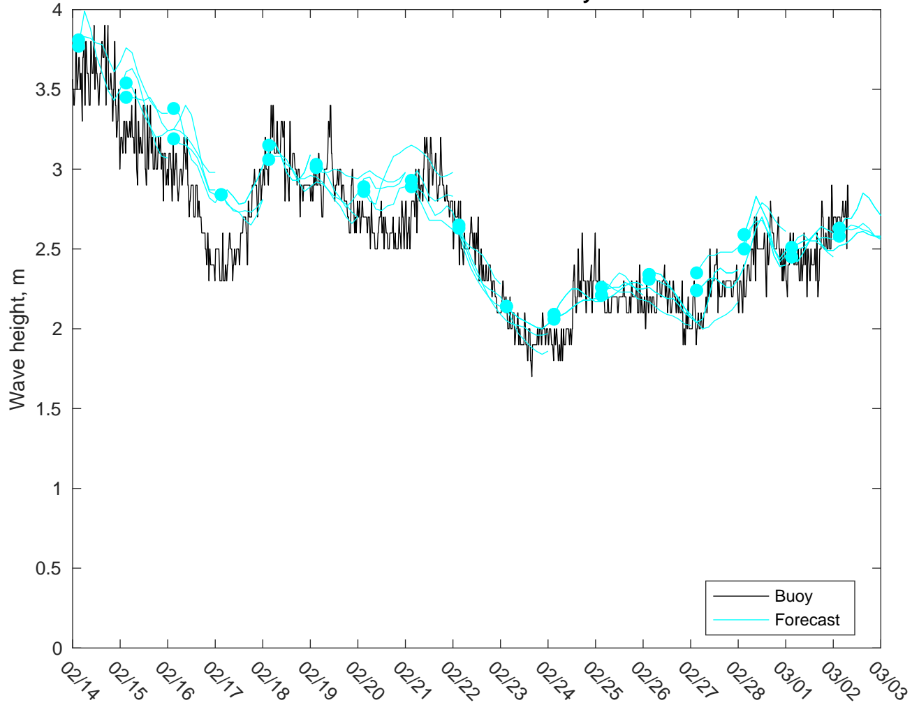
NDBC 41040 vs CMEMS Waves: 5 to 7 day forecast
