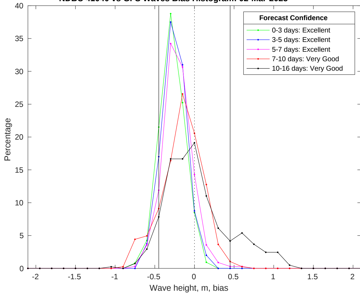
NDBC 41040 vs GFS Waves Bias Histogram: 02-Mar-2025
