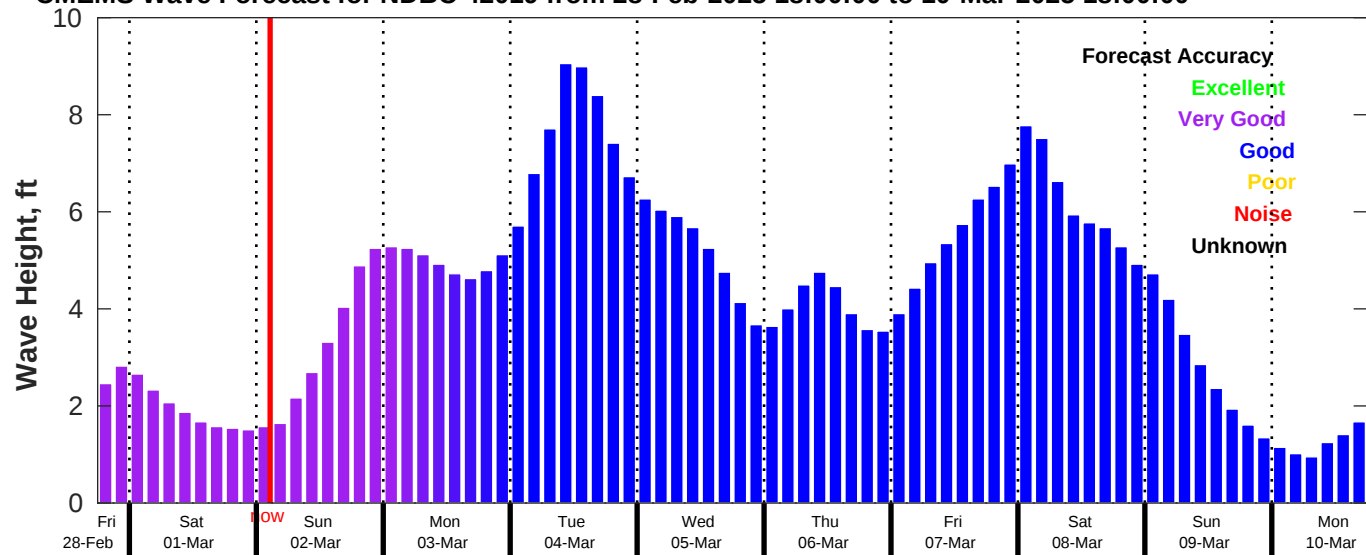
CMEMS Wave Forecast for NDBC 42019 from 28-Feb-2025 18:00:00 to 10-Mar-2025 18:00:00
