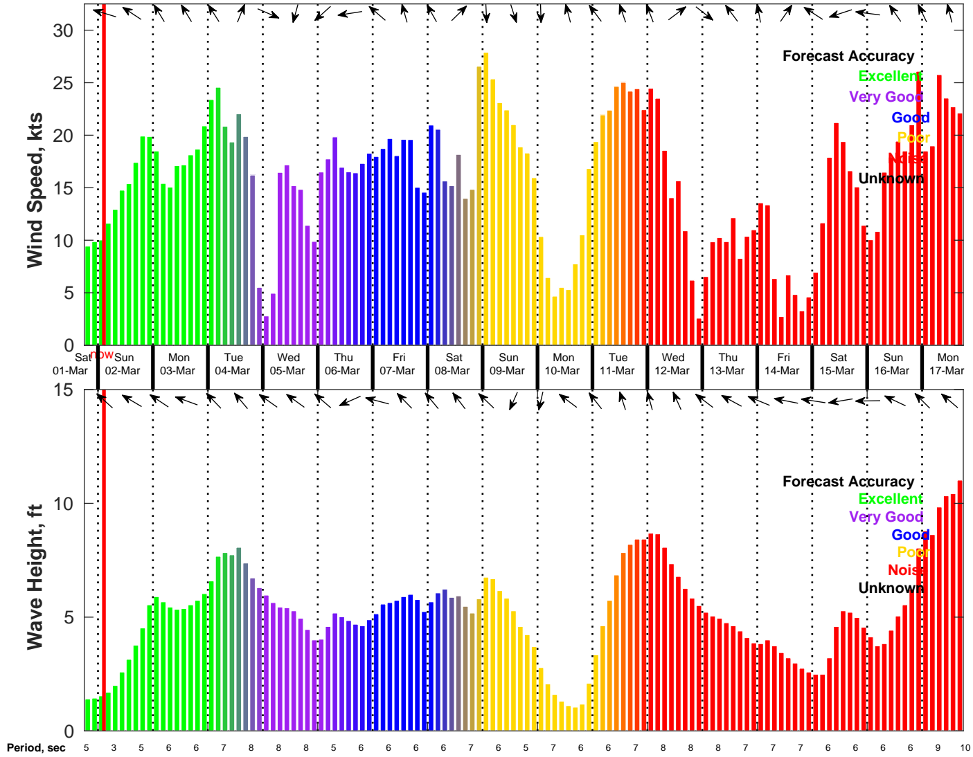
Wind & Wave Forecast for NDBC 42019 from 01-Mar-2025 18:00:00 to 17-Mar-2025 18:00:00
