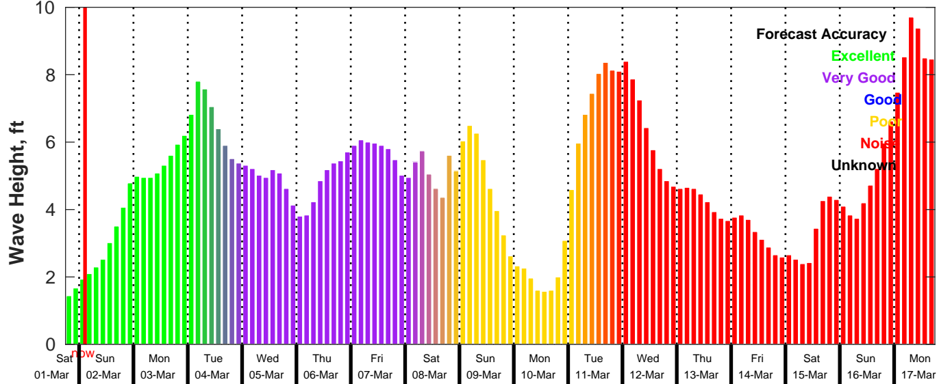
GFS Wave Forecast for NDBC 42020 from 01-Mar-2025 18:00:00 to 17-Mar-2025 18:00:00
