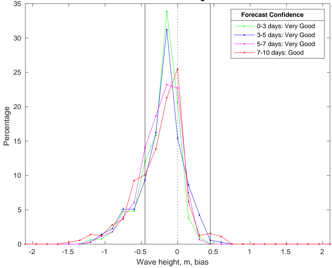
NDBC 42035 vs CMEMS Waves Bias Histogram: 02-Mar-2025
