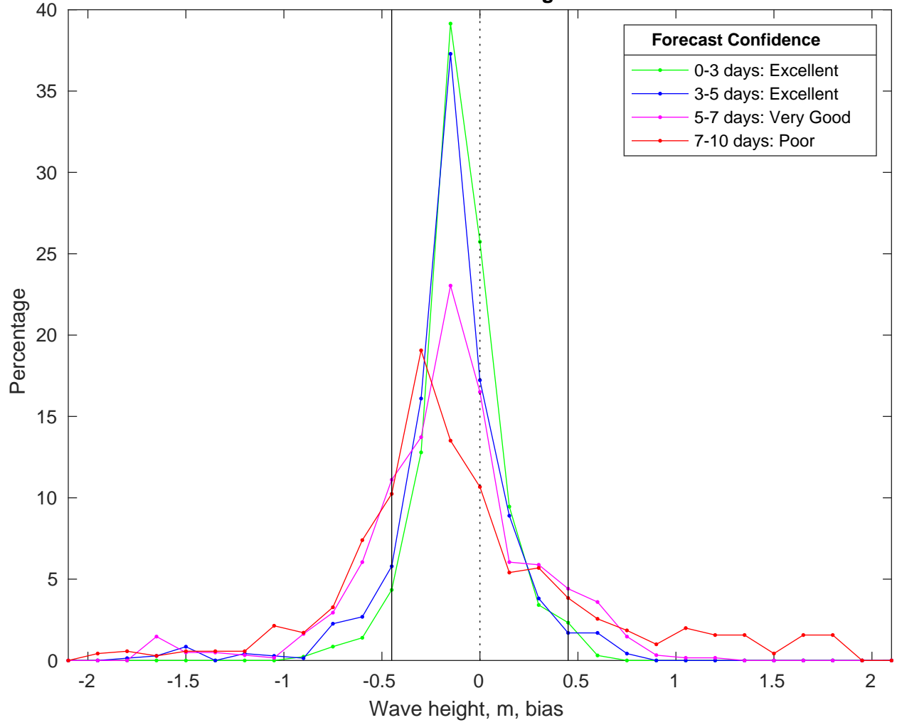
NDBC 42036 vs CMEMS Waves Bias Histogram: 02-Mar-2025
