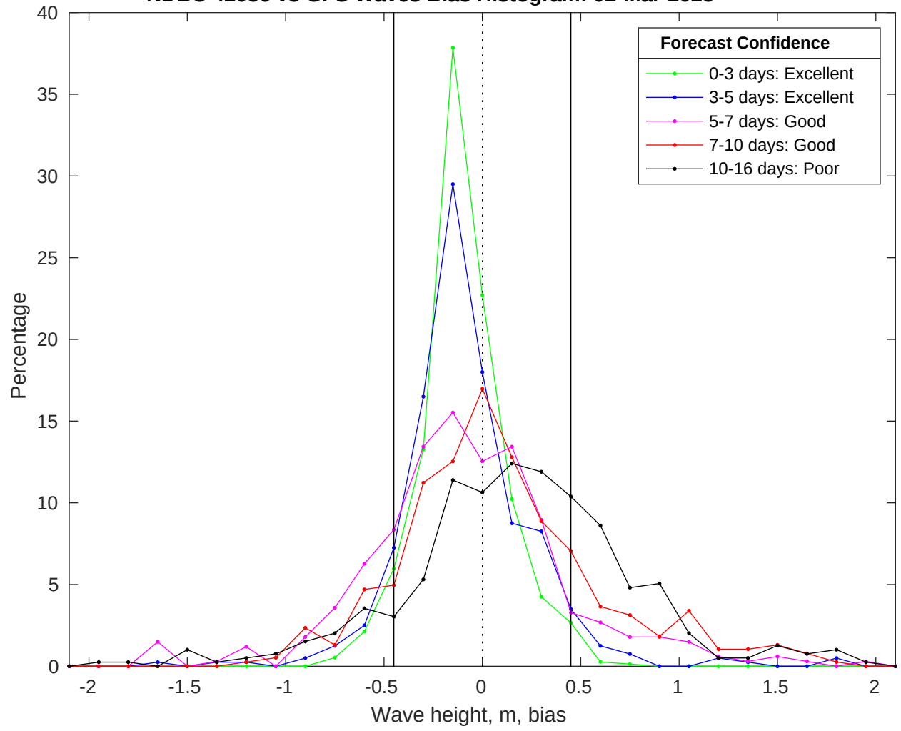
NDBC 42036 vs GFS Waves Bias Histogram: 02-Mar-2025
