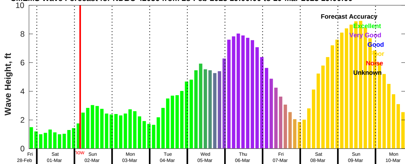
CMEMS Wave Forecast for NDBC 42036 from 28-Feb-2025 19:00:00 to 10-Mar-2025 19:00:00
