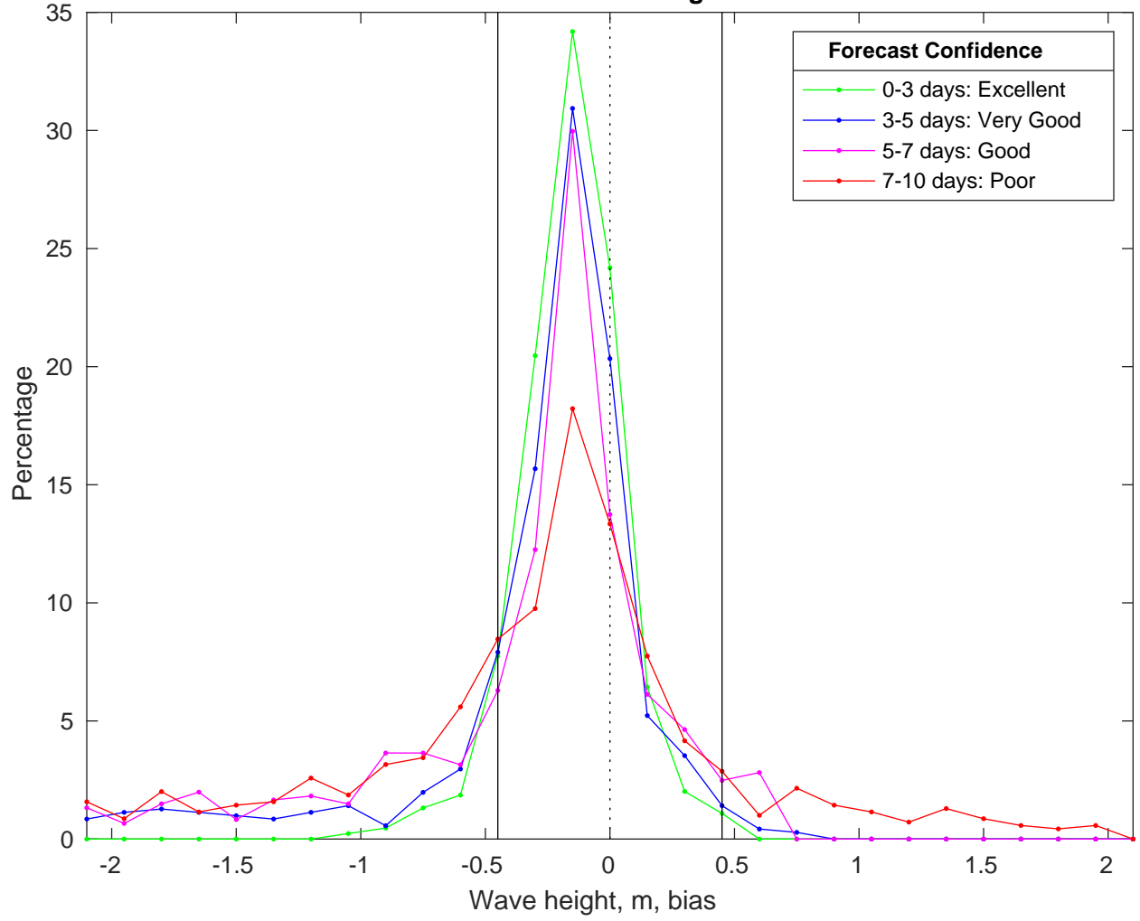
NDBC 42040 vs CMEMS Waves Bias Histogram: 02-Mar-2025
