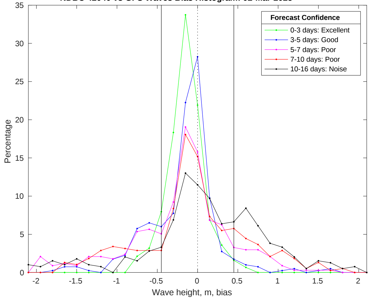
NDBC 42040 vs GFS Waves Bias Histogram: 02-Mar-2025
