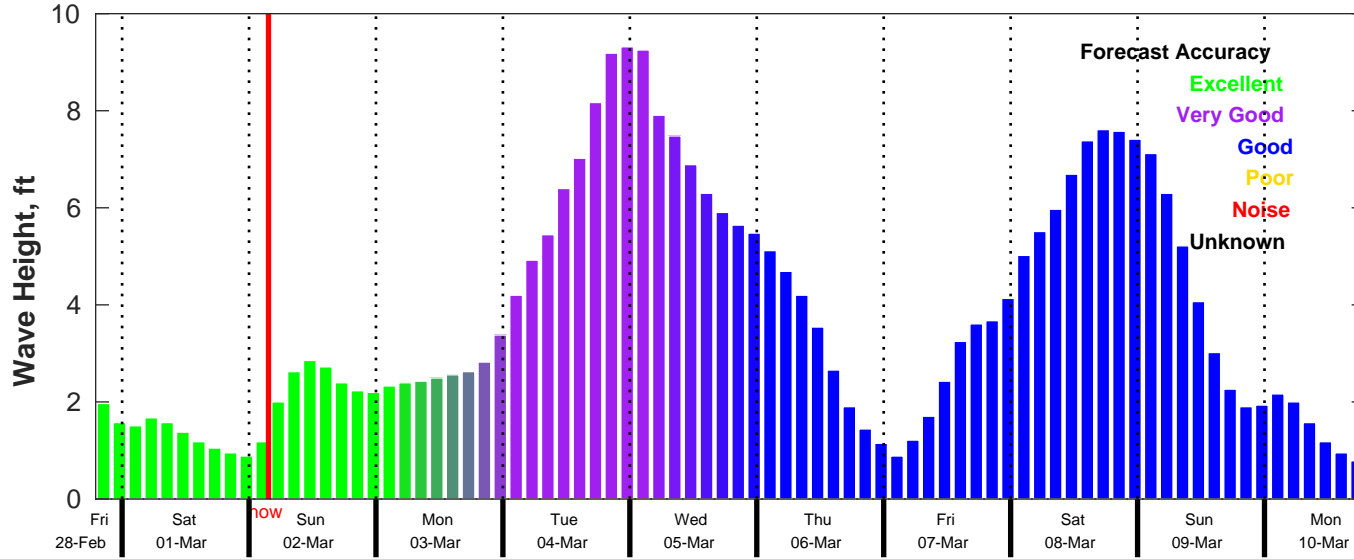
CMEMS Wave Forecast for NDBC 42084 from 28-Feb-2025 19:00:00 to 10-Mar-2025 19:00:00
