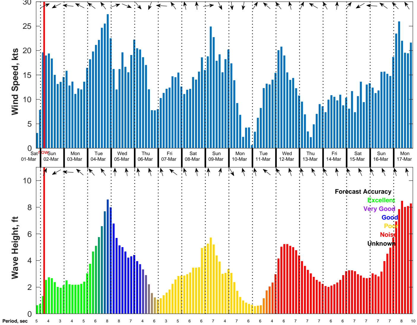
Wind & Wave Forecast for NDBC 42084 from 01-Mar-2025 19:00:00 to 17-Mar-2025 19:00:00
