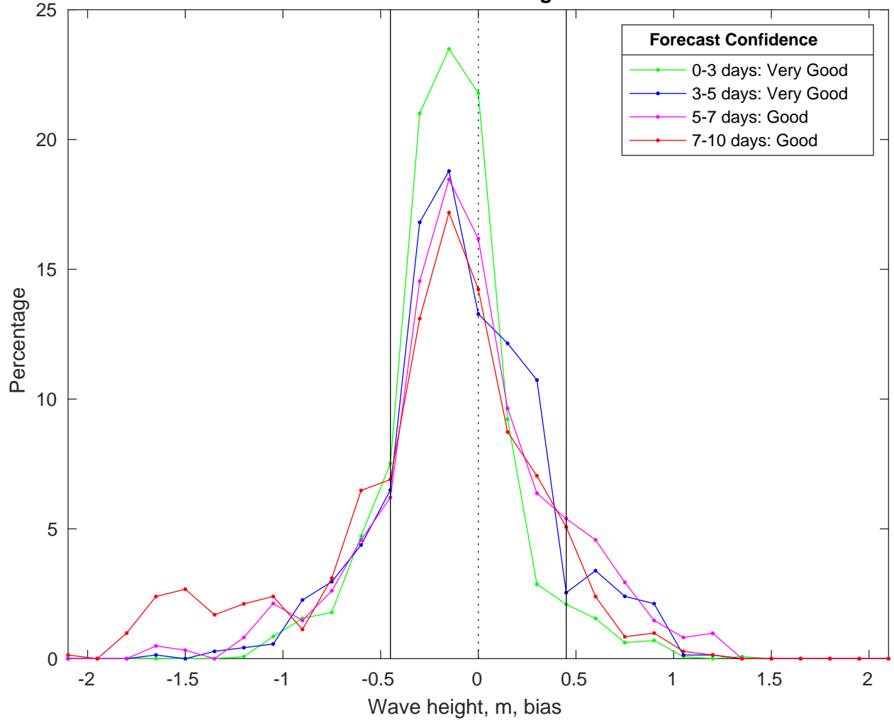
NDBC 46011 vs CMEMS Waves Bias Histogram: 02-Mar-2025
