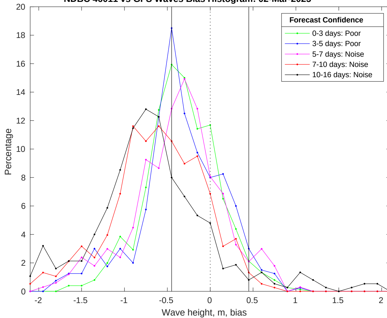
NDBC 46011 vs GFS Waves Bias Histogram: 02-Mar-2025
