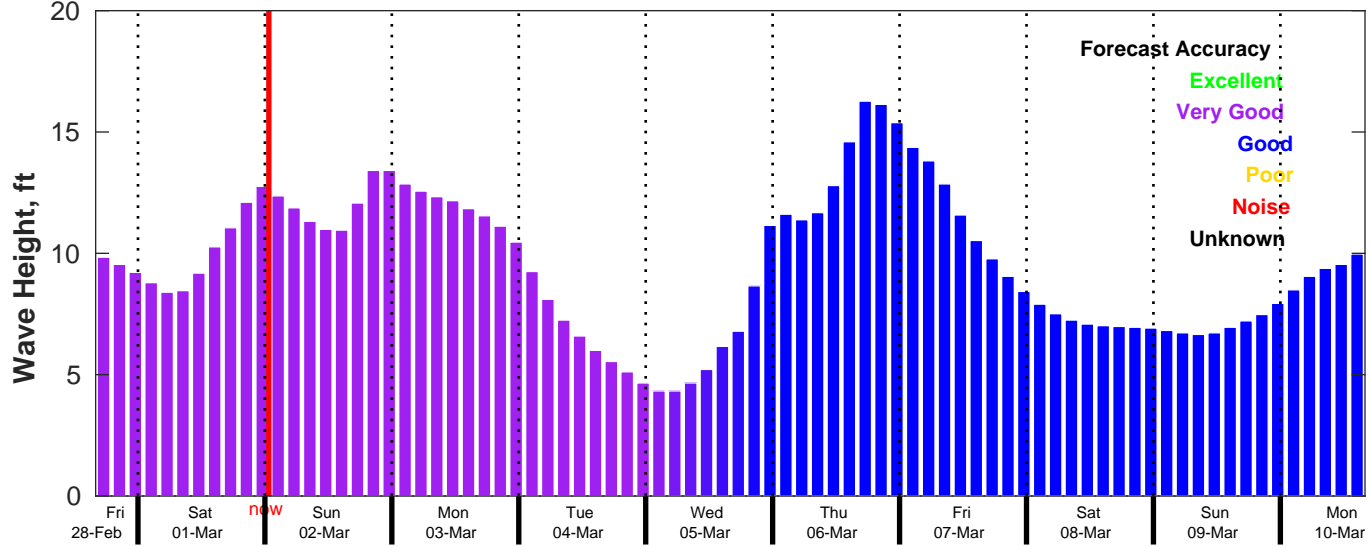
CMEMS Wave Forecast for NDBC 46011 from 28-Feb-2025 16:00:00 to 10-Mar-2025 16:00:00
