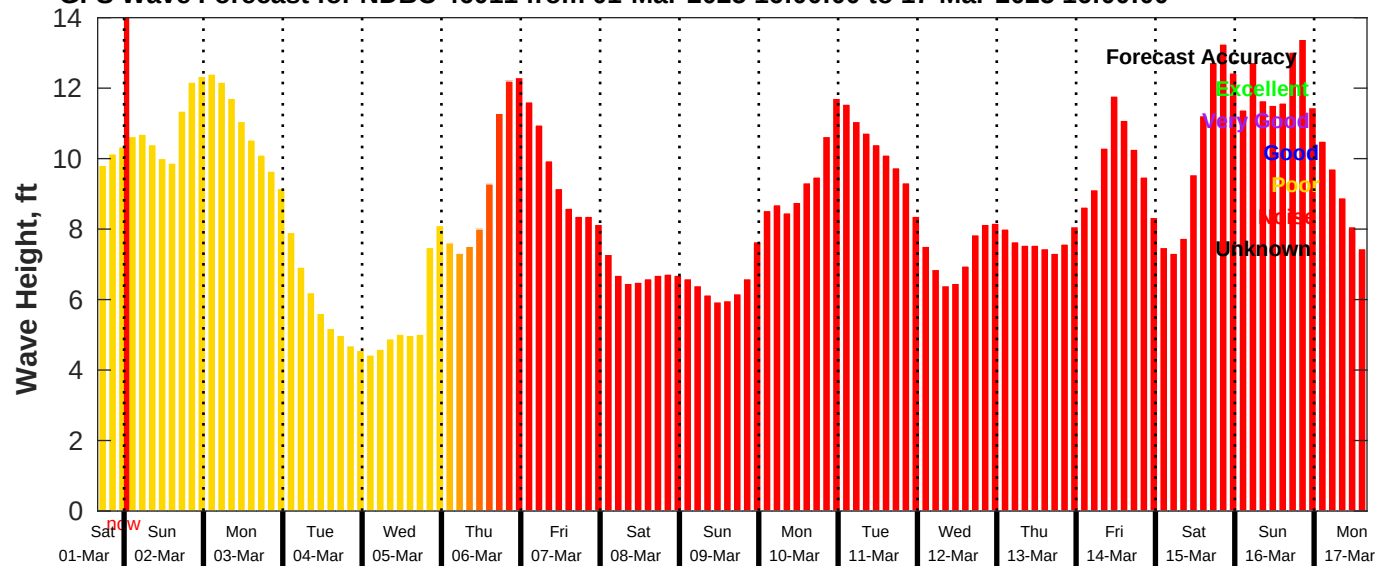
GFS Wave Forecast for NDBC 46011 from 01-Mar-2025 16:00:00 to 17-Mar-2025 16:00:00
