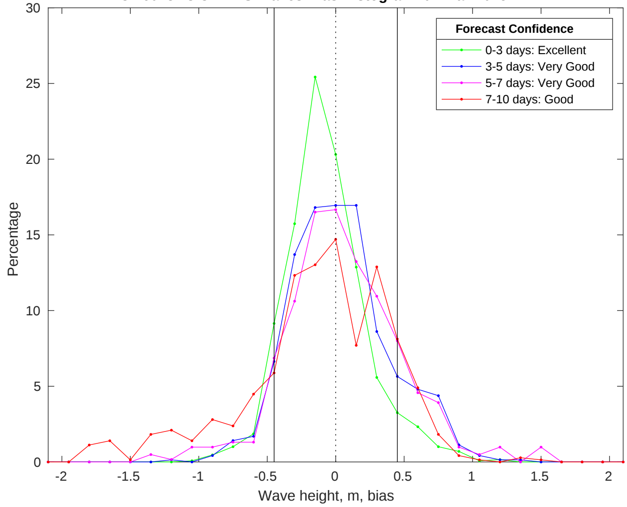
NDBC 46028 vs CMEMS Waves Bias Histogram: 02-Mar-2025
