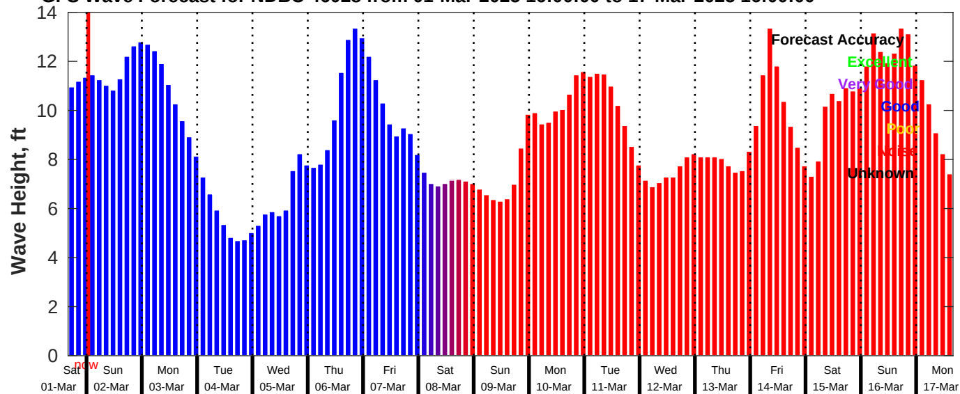
GFS Wave Forecast for NDBC 46028 from 01-Mar-2025 16:00:00 to 17-Mar-2025 16:00:00
