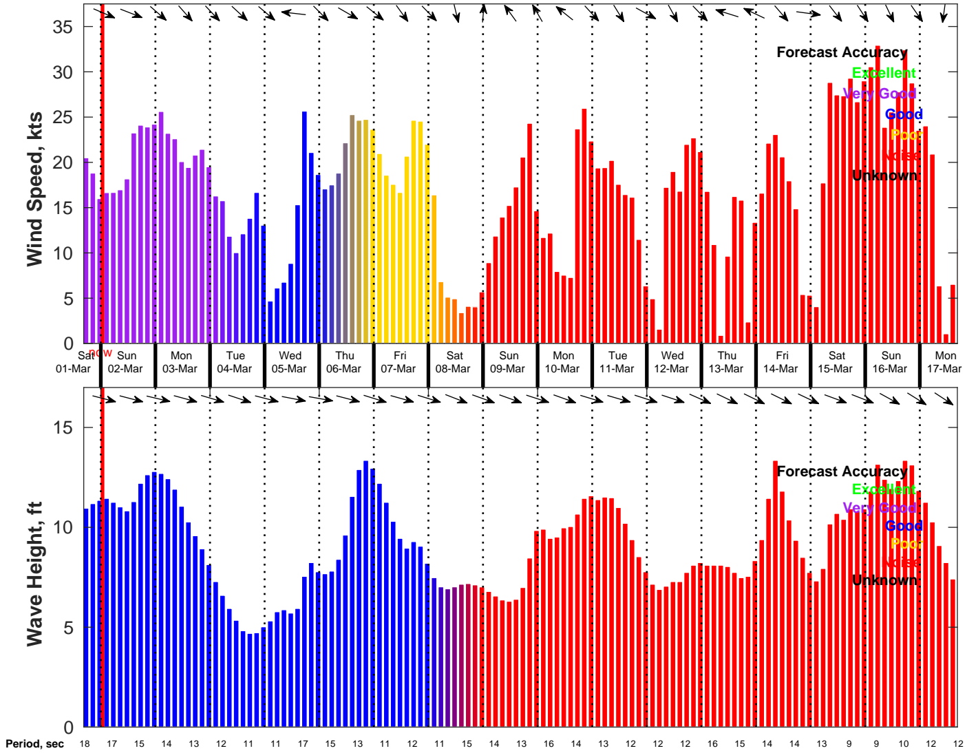
Wind & Wave Forecast for NDBC 46028 from 01-Mar-2025 16:00:00 to 17-Mar-2025 16:00:00
