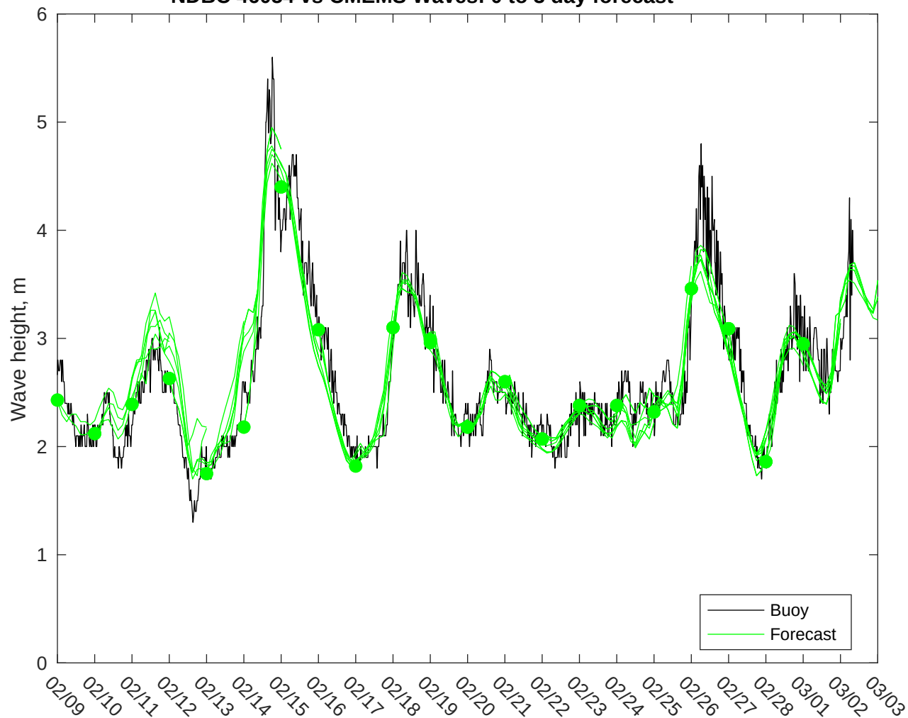
NDBC 46054 vs CMEMS Waves: 0 to 3 day forecast
