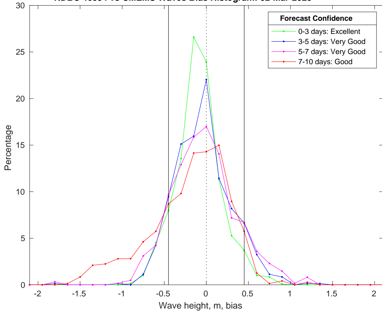
NDBC 46054 vs CMEMS Waves Bias Histogram: 02-Mar-2025
