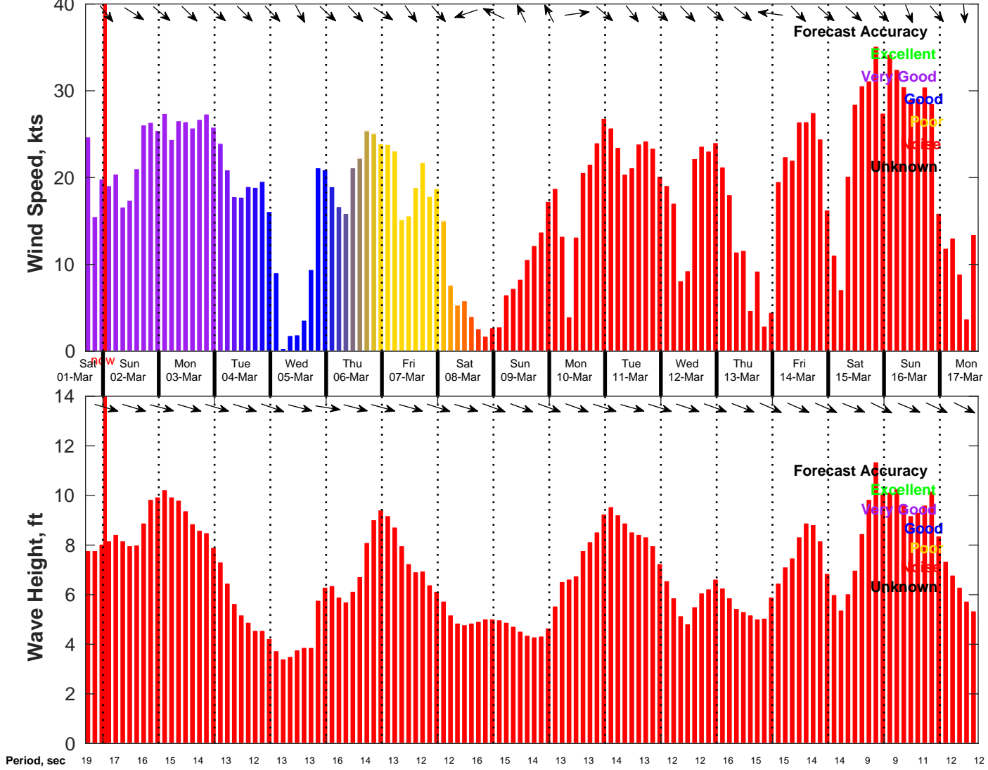
Wind & Wave Forecast for NDBC 46054 from 01-Mar-2025 16:00:00 to 17-Mar-2025 16:00:00
