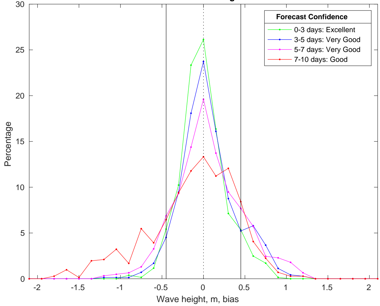
NDBC 46069 vs CMEMS Waves Bias Histogram: 02-Mar-2025
