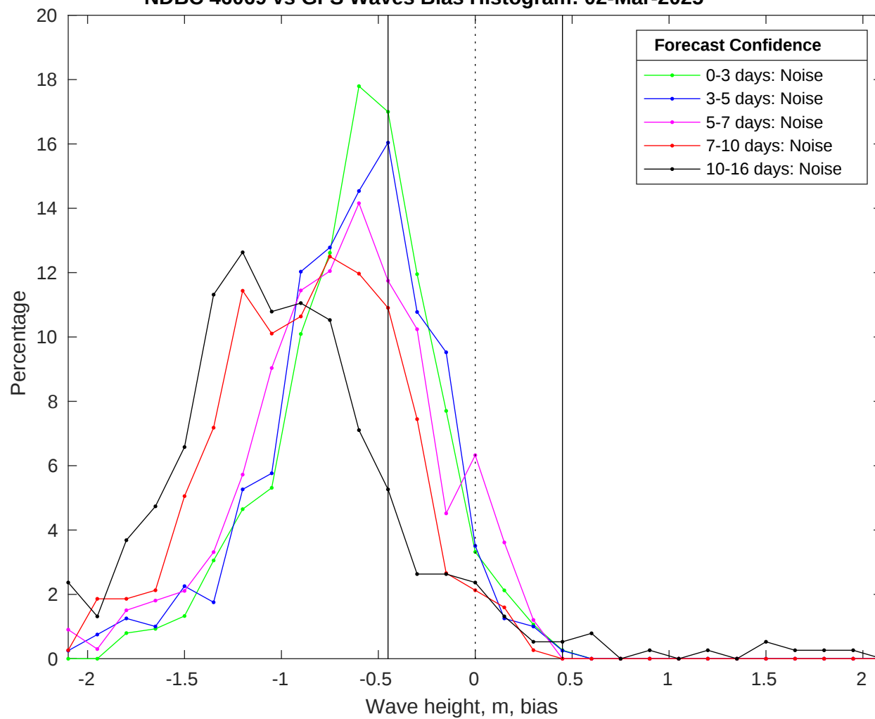
NDBC 46069 vs GFS Waves Bias Histogram: 02-Mar-2025
