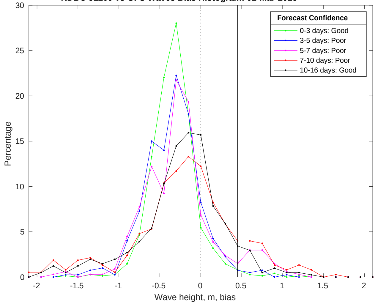
NDBC 51209 vs GFS Waves Bias Histogram: 02-Mar-2025
