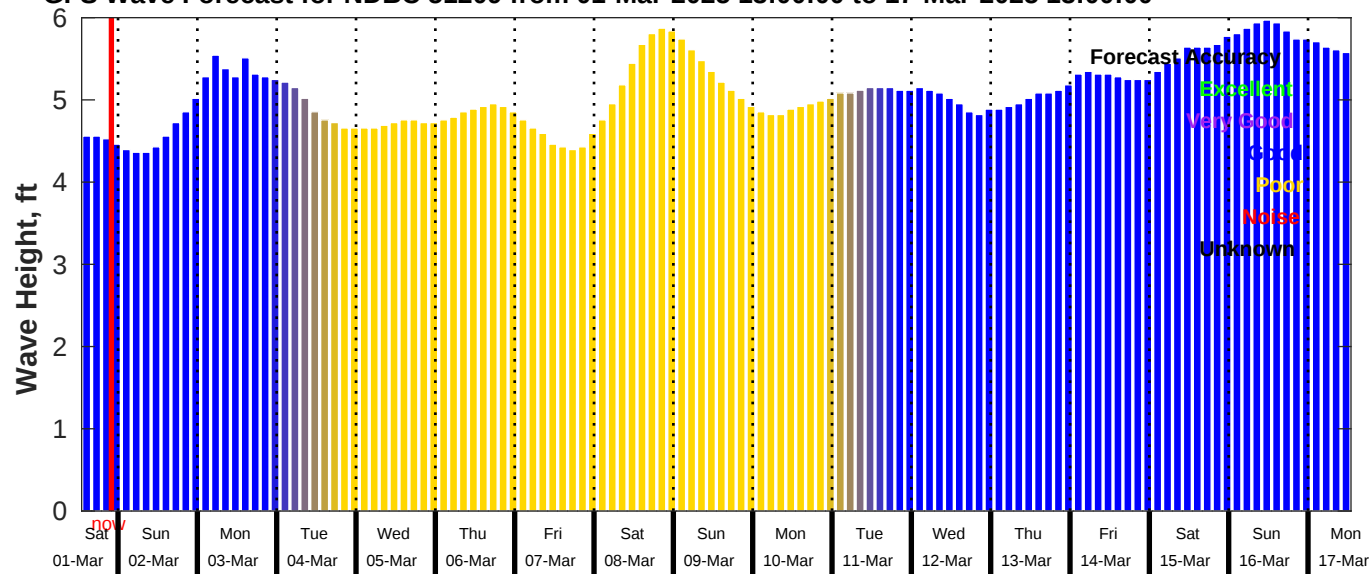
GFS Wave Forecast for NDBC 51209 from 01-Mar-2025 13:00:00 to 17-Mar-2025 13:00:00
