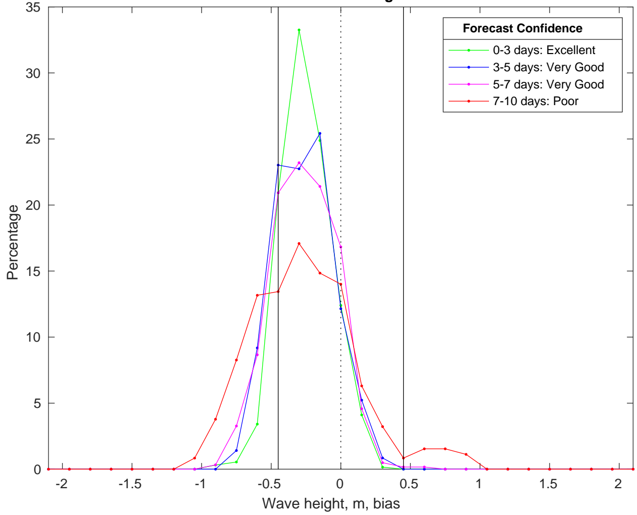
NDBC 52211 vs CMEMS Waves Bias Histogram: 02-Mar-2025
