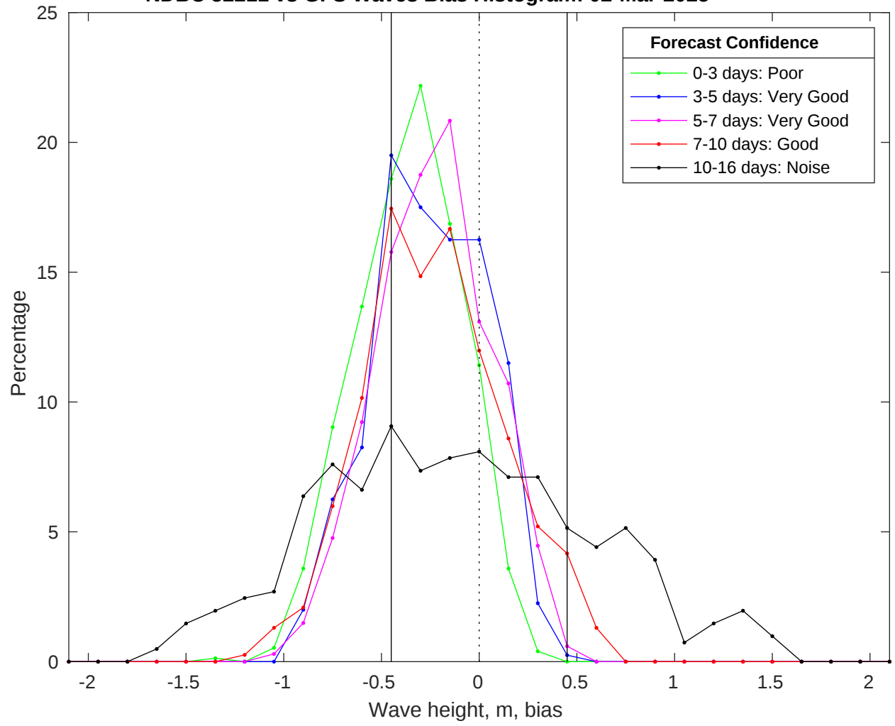
NDBC 52211 vs GFS Waves Bias Histogram: 02-Mar-2025
