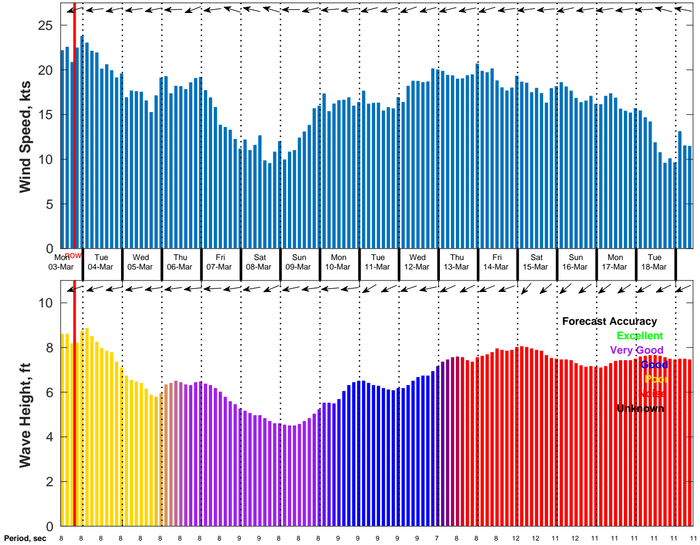
Wind & Wave Forecast for NDBC 52211 from 02-Mar-2025 10:00:00 to 18-Mar-2025 10:00:00
