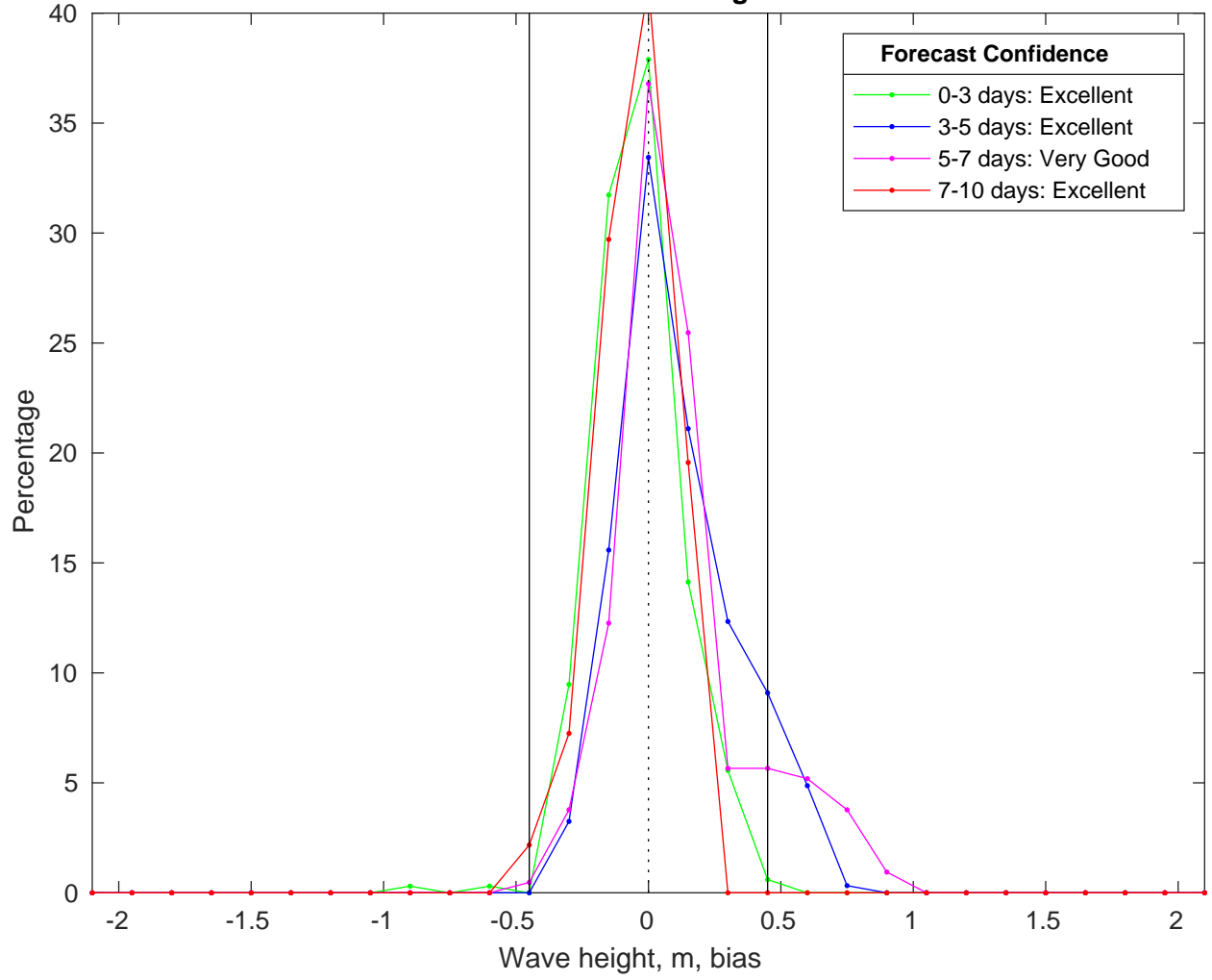
NDBC 52212 vs CMEMS Waves Bias Histogram: 02-Mar-2025
