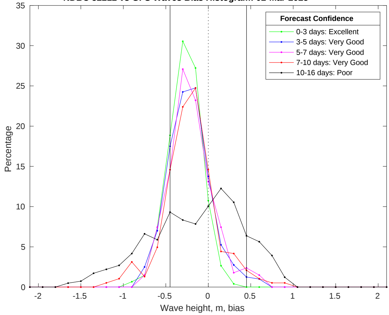
NDBC 52212 vs GFS Waves Bias Histogram: 02-Mar-2025
