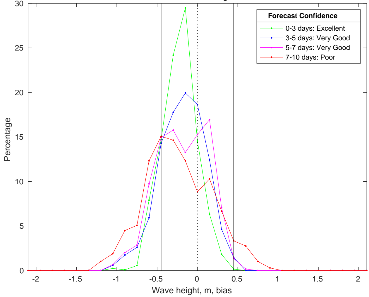
NDBC 52213 vs CMEMS Waves Bias Histogram: 02-Mar-2025
