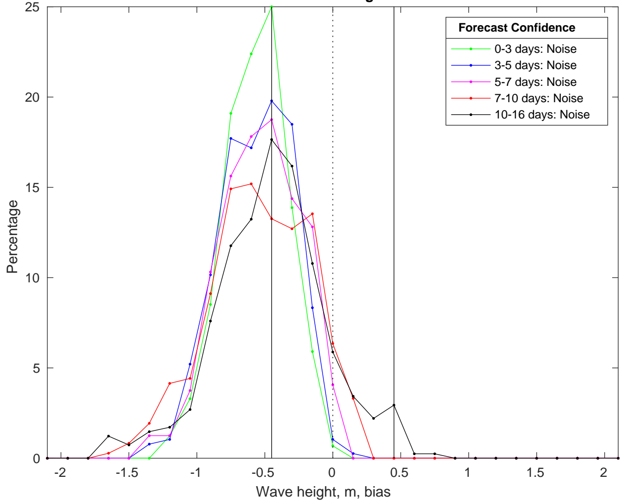
NDBC 52213 vs GFS Waves Bias Histogram: 02-Mar-2025
