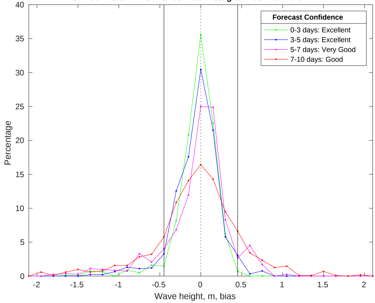
NDBC 41004 vs CMEMS Waves Bias Histogram: 03-Mar-2025
