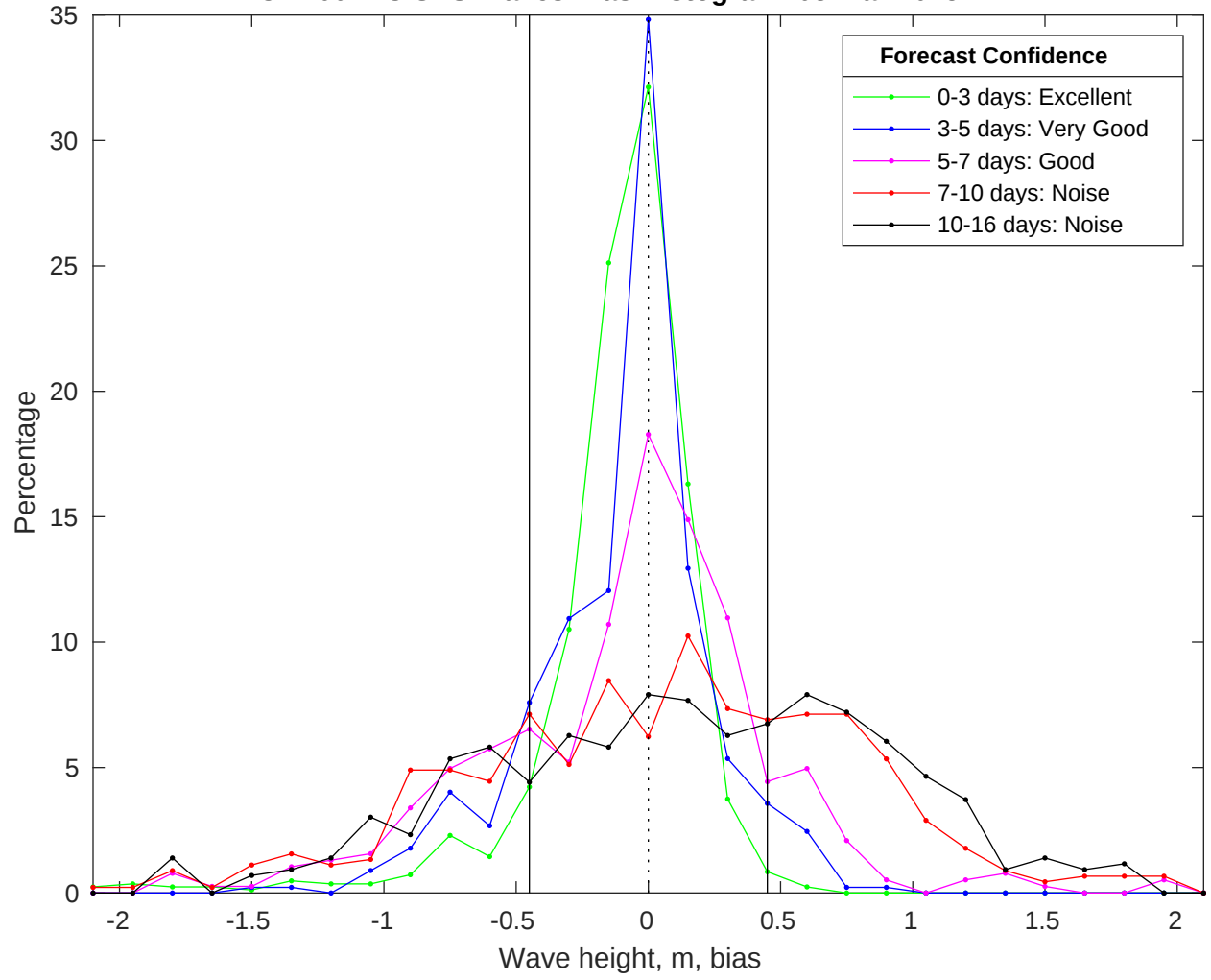
NDBC 41004 vs GFS Waves Bias Histogram: 03-Mar-2025
