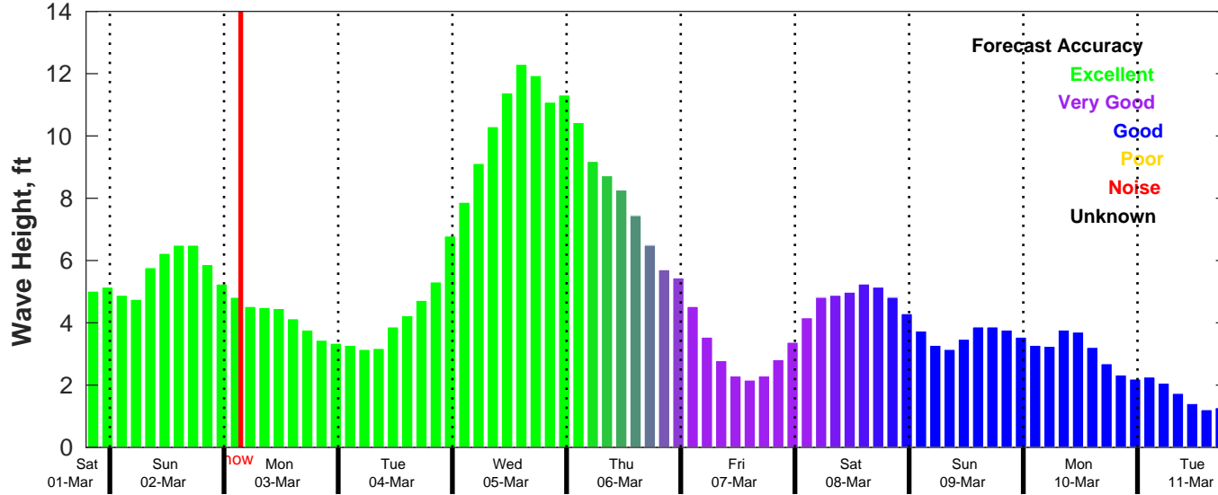
CMEMS Wave Forecast for NDBC 41004 from 01-Mar-2025 19:00:00 to 11-Mar-2025 19:00:00
