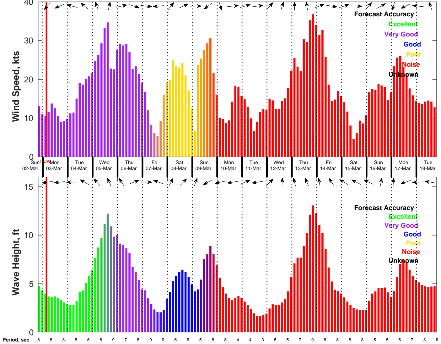
Wind & Wave Forecast for NDBC 41004 from 02-Mar-2025 19:00:00 to 18-Mar-2025 19:00:00
