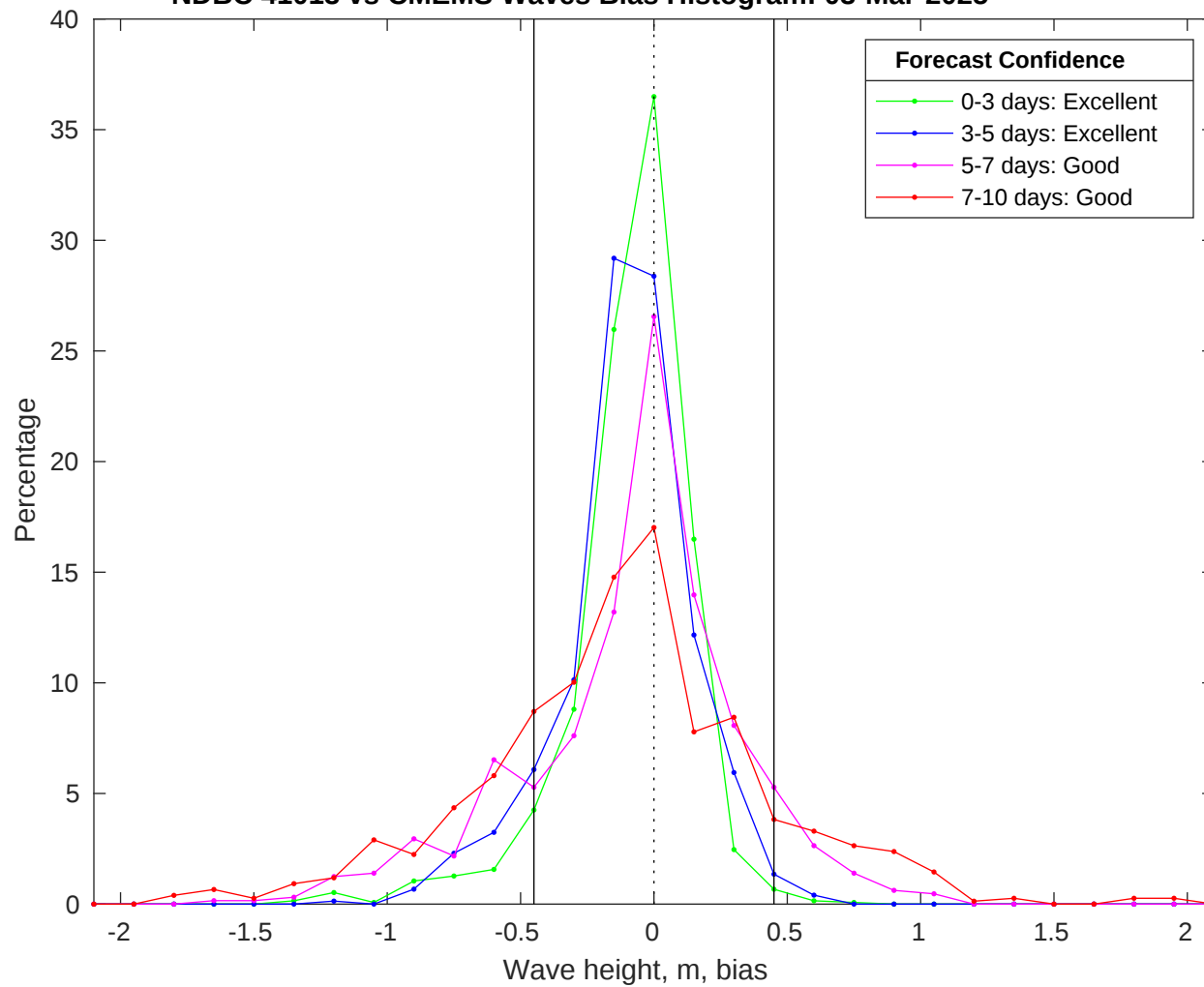
NDBC 41013 vs CMEMS Waves Bias Histogram: 03-Mar-2025
