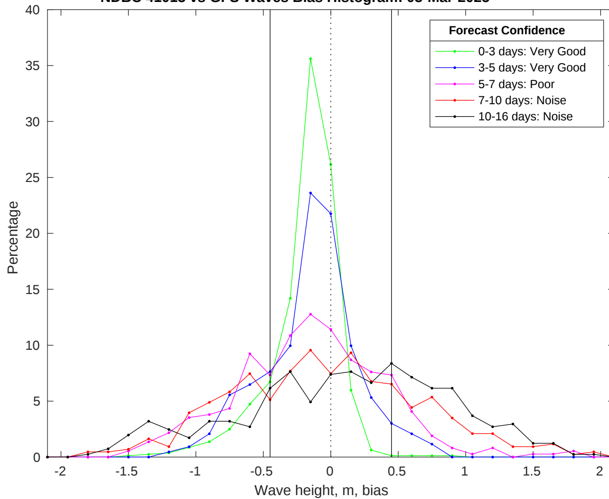
NDBC 41013 vs GFS Waves Bias Histogram: 03-Mar-2025
