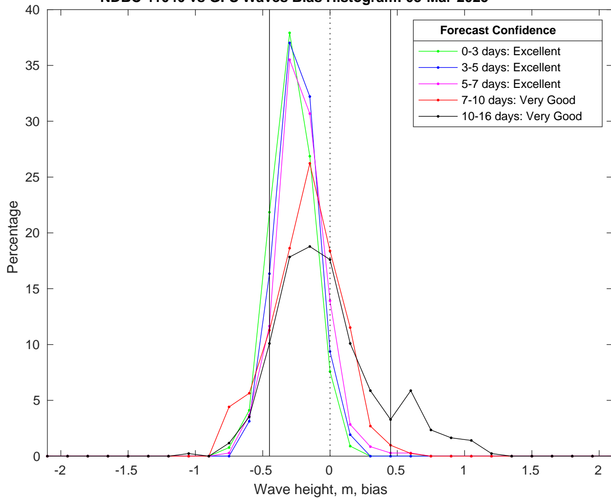
NDBC 41040 vs GFS Waves Bias Histogram: 03-Mar-2025
