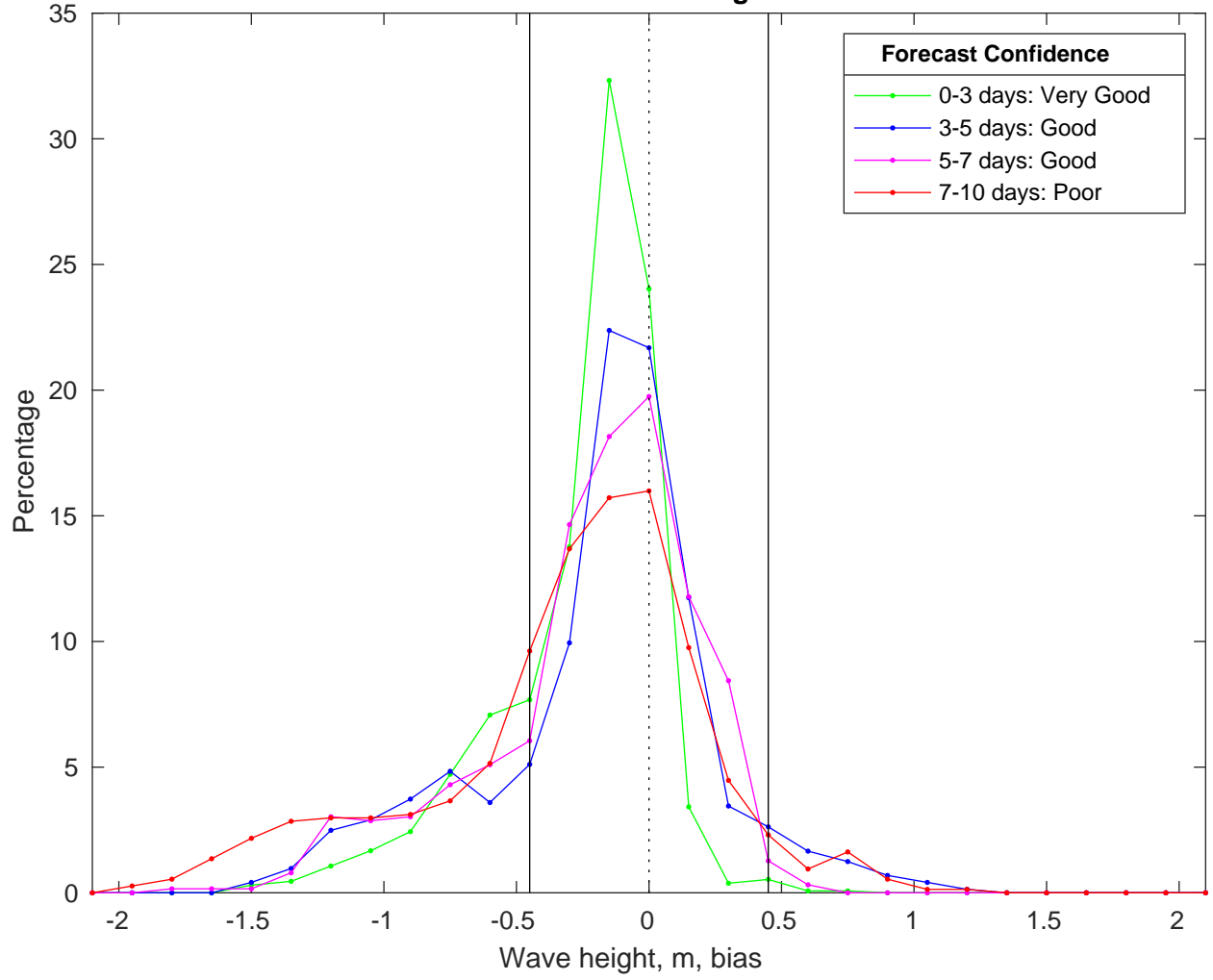
NDBC 42019 vs CMEMS Waves Bias Histogram: 03-Mar-2025
