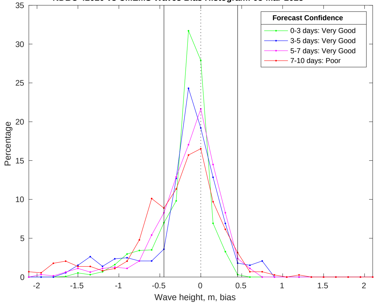
NDBC 42020 vs CMEMS Waves Bias Histogram: 03-Mar-2025
