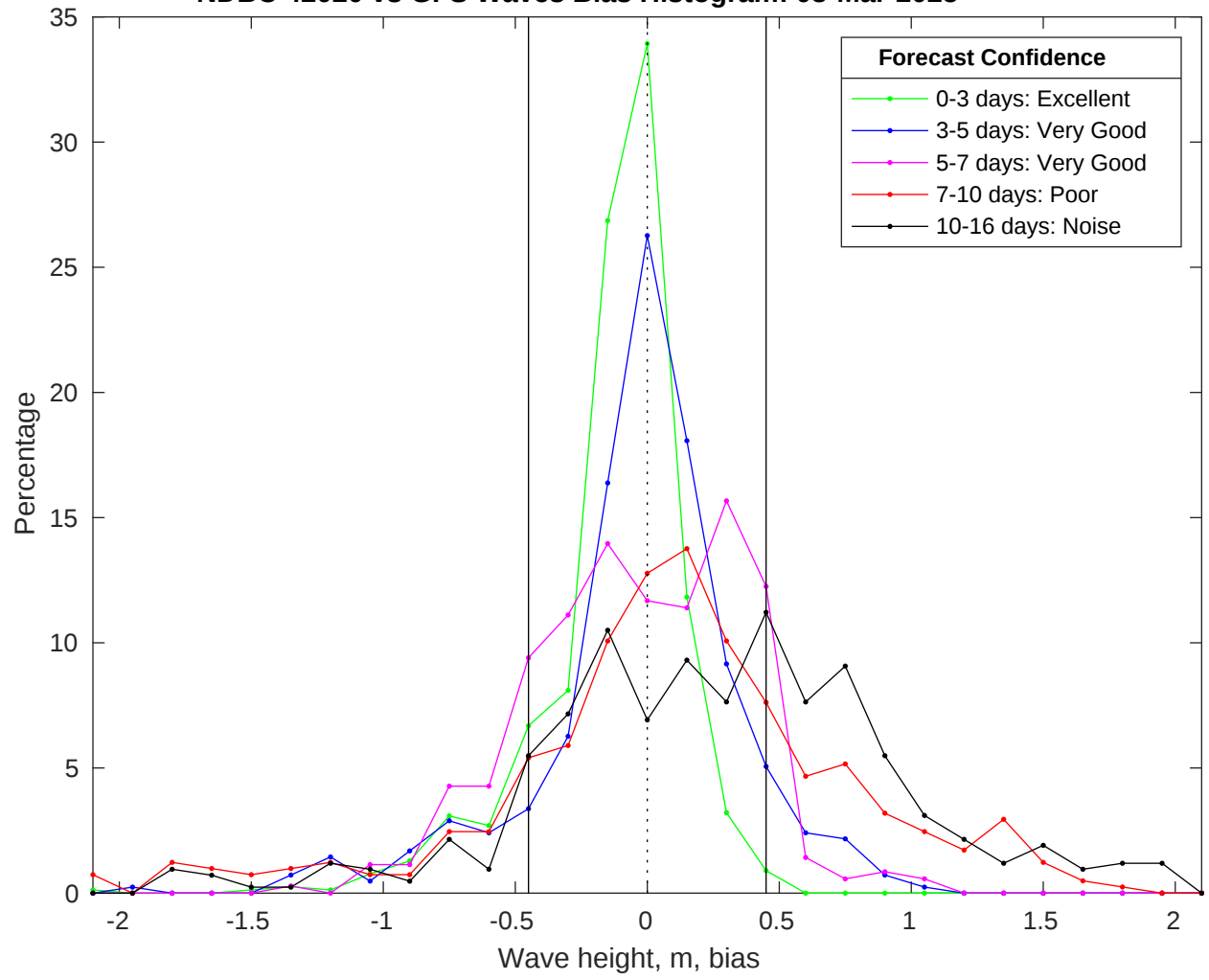
NDBC 42020 vs GFS Waves Bias Histogram: 03-Mar-2025
