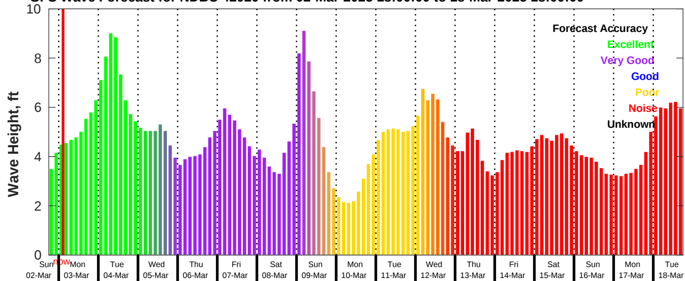
GFS Wave Forecast for NDBC 42020 from 02-Mar-2025 18:00:00 to 18-Mar-2025 18:00:00
